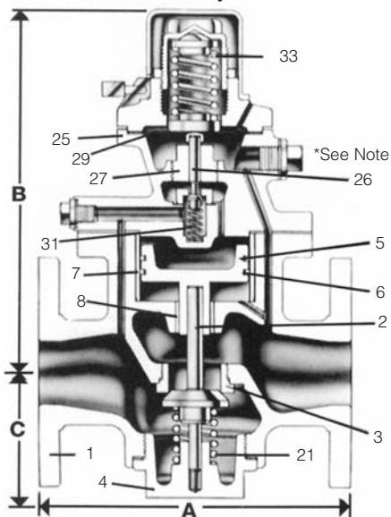
Standard Assembly
